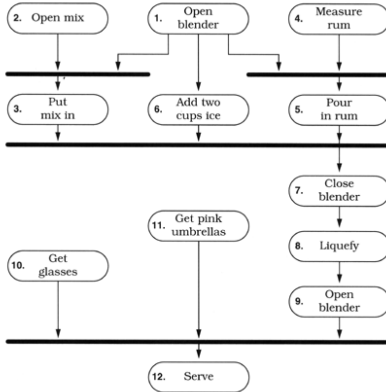
Figure 5.2. UML activity diagram: making a piña colada
