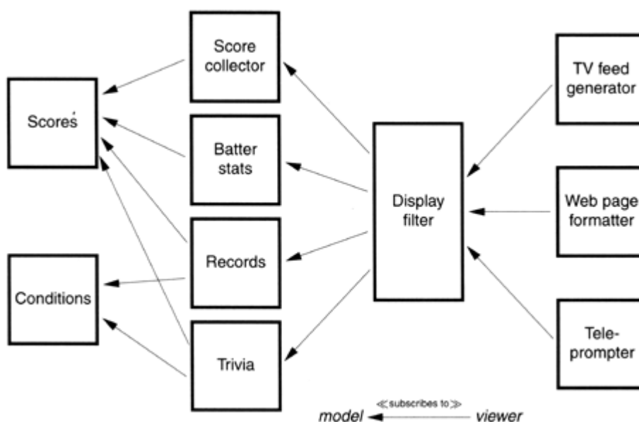
Figure 5.5. Baseball reporting, Viewers subscribe to models.
